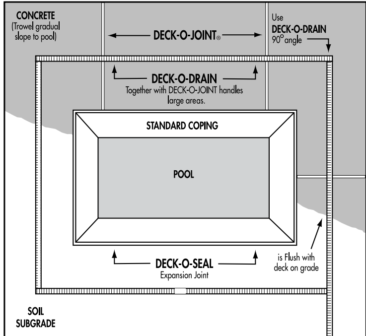
TYPICAL POOL DECK APPLICATION FIGURE #1(TOP VIEW)
